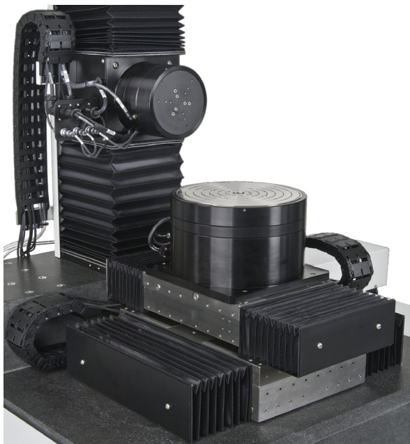
ABTech 5 axis air bearing optical metrology platform
